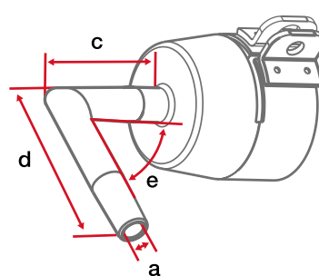
Soldering nozzle \varnothing 21.3 mm
